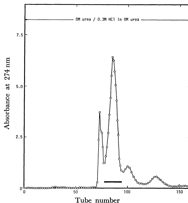
Fig. 4. Chromatogram of the S -sulfonate of Leu-Glu-Gly-Pro-Pro-Gln-Lys[Z(2-Cl)]-Arg-A-chain on DEAE-Sephadex A-25 under the conditions described in the text.
